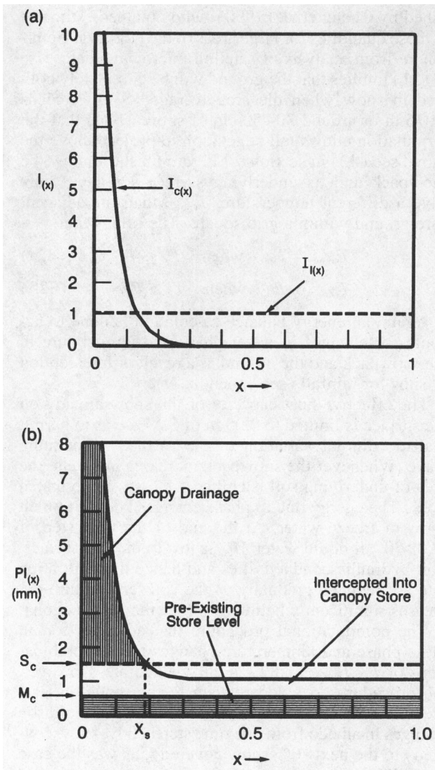
FIG. 5. (a) Precipitation area-amount relationships used in SiB2. The variable x refers to fraction of the grid area, the variable I(x) refers to the relative amount of precipitation. Note that the large-scale precipitation I_l(x) is almost invariant over the grid area, while convective precipitation I_c(x) is nonuniformly distributed. (b) Dynamics of precipitation interception by a vegetation canopy in SiB2. The amount of water already stored in the canopy prior to rainfall interception, M_{cs} + M_{cw} , is considered to be uniformly distributed over the grid area (see horizontally hatched area). The integral of the water amount above M_{cs} + M_{cw} represents the total amount of water intercepted by the canopy. Here x_s is the proportion of the grid area where the intercepted rainfall plus the preexisting canopy water storage, M_{cs} + M_{cw} , exceeds the canopy storage limit S_c . All water above the S_c limit drains off the canopy to form D_c (vertically hatched area), all below it is added to the canopy interception store.
