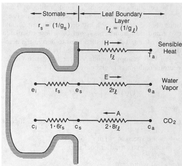
FIG. 4. Coupled leaf stomatal photosynthesis–conductance models as described by Collatz et al. (1991). System shows pathways for heat, \text{CO}_2 , and water vapor flux (reproduced from Sellers et al. 1992a). Term r_l refers to the two-sided leaf laminar boundary-layer resistance for sensible heat; water and \text{CO}_2 are assumed to be lost from one side of the leaf only; r_b is the canopy integral of r_l ; and r_c is the canopy integral of r_s .
