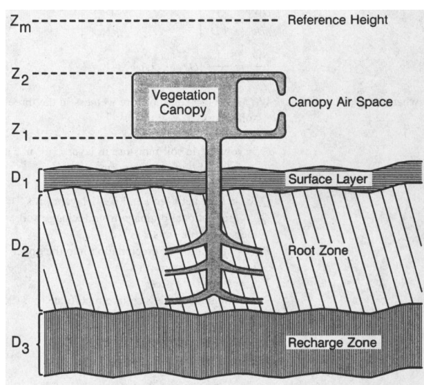
FIG. 1. Structure of the SiB2 model. SiB2 has only one vegetation layer, while SiB1 had provision for upper story and ground cover vegetation.
