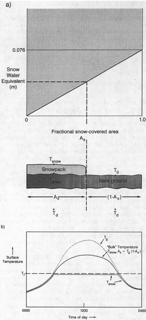
FIG. 6. (a) Relationship between SWE and snow extent over a grid area as modeled in SiB2, based on data published by Chang et al. (1990). (b) Diurnal cycle of ground and snowpack temperature for a patchy snow cover as represented by SiB2. Note that the combined effective temperature, T_B = T_{snow}A_s + T_g(1 - A_s) , is used for aerodynamic and radiation exchange calculations.
